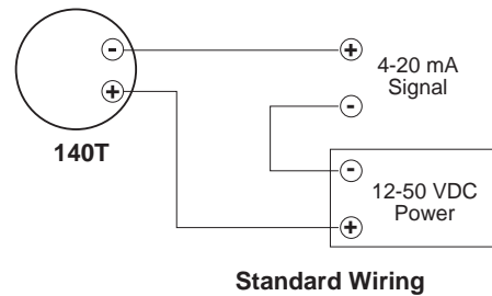
Standard Wiring
